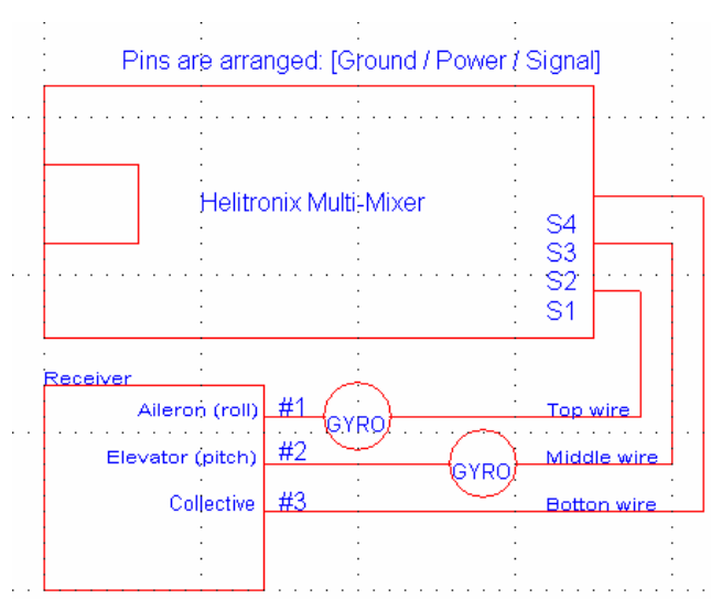
Figure 1 - Schematic Diagram of Receiver Connections
