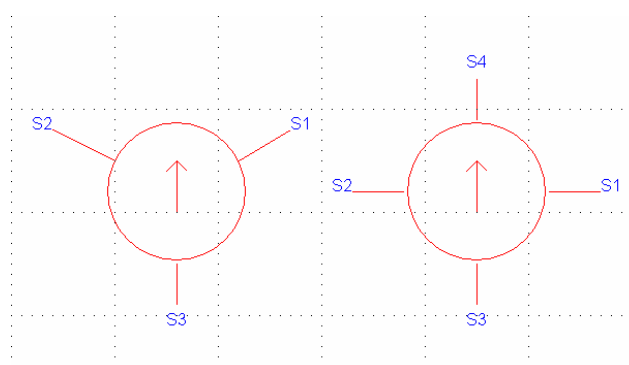
Figure 2 - Servo layout for 3 and 4 servo CCPM washplate configuration
